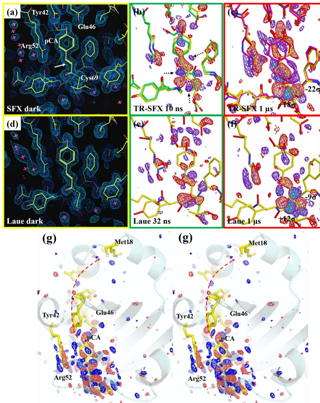
Figure 3.2. Yellow lines in all maps: dark state model. (a) TR-SFX electron density map of dark state model ( 1.1\sigma contour level) to a resolution of 1.6 \text{ \AA} . The pCA chromophore and some surrounding residues are labeled. White arrow: location of the C2=C3 double bond. (b) TR-SFX DED map for 10 ns time-delay; green lines: structure of the I_{CT} intermediate; dashed arrows: features that belong to other intermediates not shown here. (c) 1 \mu\text{s} time-delay, TR-SFX DED map; pink lines: pR1 intermediate; red lines: pR2 intermediate. (d) TR-LX electron density map of dark state model ( 1.1\sigma contour level) to a resolution of 1.6 \text{ \AA} . (e) The 32 ns time-delay, TR-LX DED map and I_{CT} structure corresponds best with 10 ns TR-SFX I_{CT} intermediate. (f) 1 \mu\text{s} TR-LX DED map. Note the high level of reaction initiation for TR-SFX. (g) Stereo view of 1 \mu\text{s} TR-SFX map overlaid on dark state model. Dashed red arrow: DED features extend to Met18; Contour levels: (b) red/blue -3\sigma/+3\sigma (c) red/white -3\sigma/-4\sigma and blue/cyan +3\sigma/+5\sigma (g) red/blue -3\sigma/+3\sigma . Panels modified from Tenboer et al. 2014.
