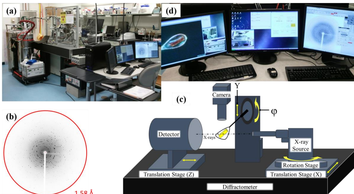
Figure 2.9. SBL1. (a) SBL1 setup in the lab. (b) Diffraction data from PYP obtained using SBL1. The red circle identifies 1.58 Å resolution. (c) A schematic of SBL1 is shown here; the sample is yellow and placed into the X-ray beam; the direction of movement for the translation and rotation stages are denoted by yellow arrows. (d) SBL1 control desk showing an experiment in progress.
